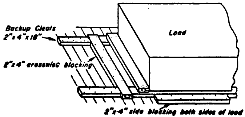
Figure 6. Floor blocking.
