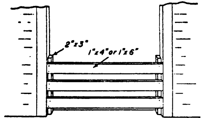
Flush Doorway Protection for Cars With Wooden Doorposts
