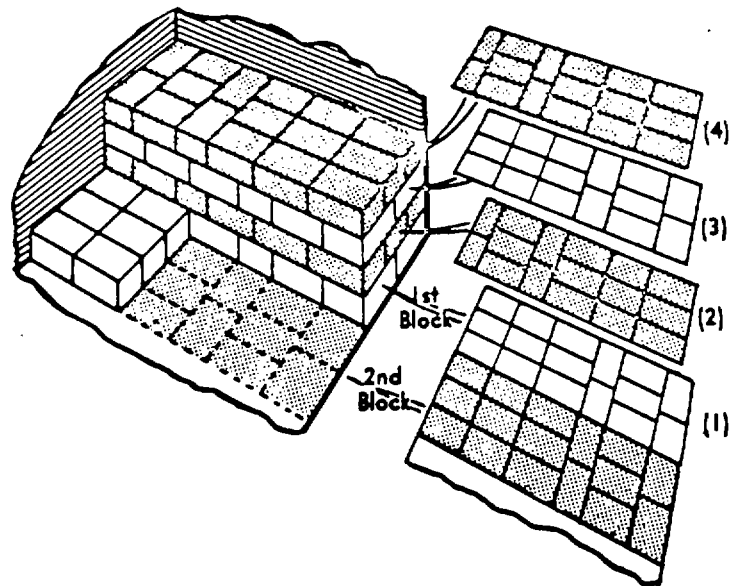
Figure 65. Bonded block pattern A.
