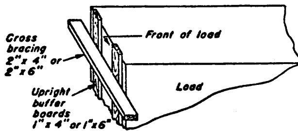
Figure 14. Cross bracing.
