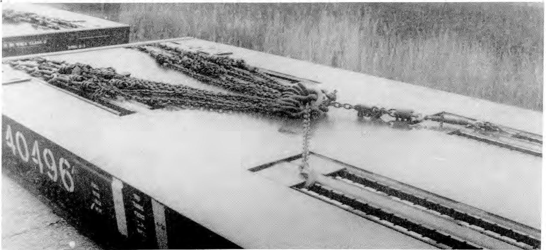
Figure 2-5. Assembly D.
