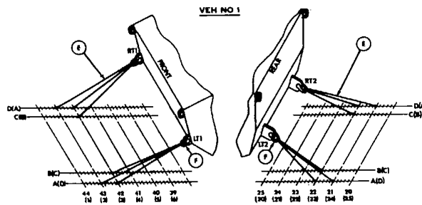
Figure 7-2. Chain tiedown arrangement for two MA109 howitzers.
